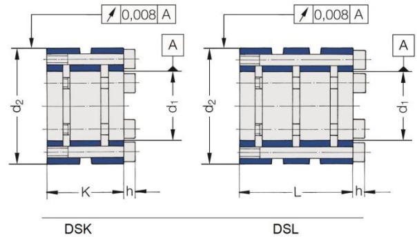
Fig. 3: Sectional view
